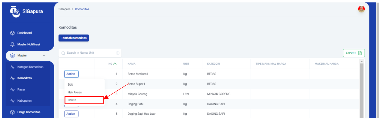
Gambar 3.24. Delete Komoditas
