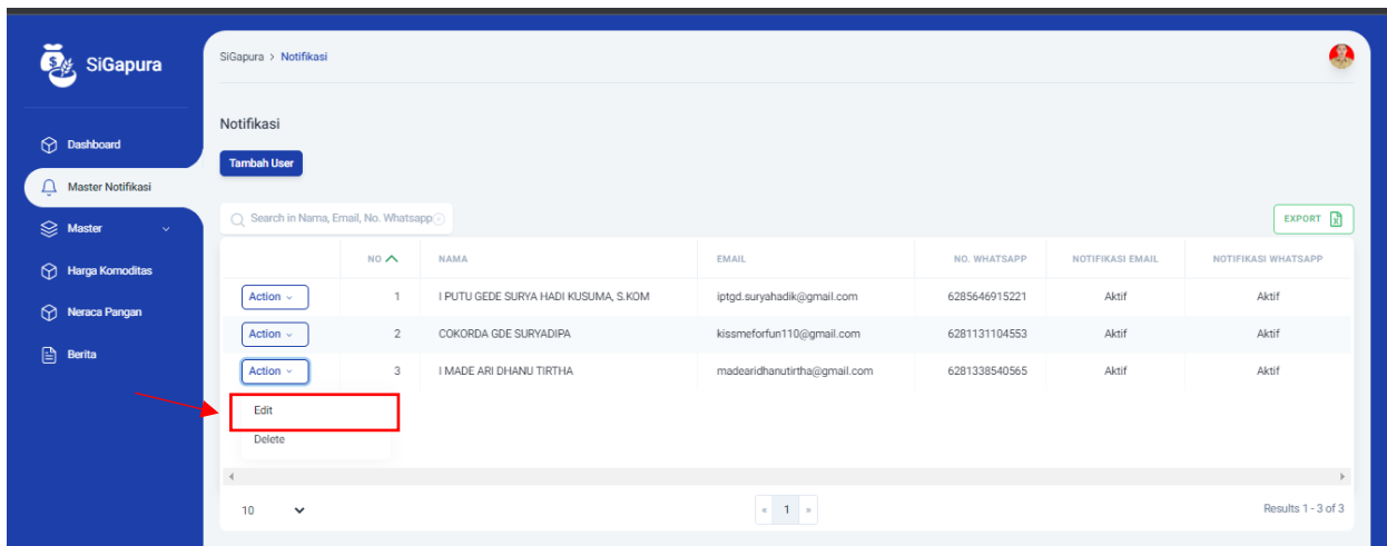
Gambar 3.6. Edit User
