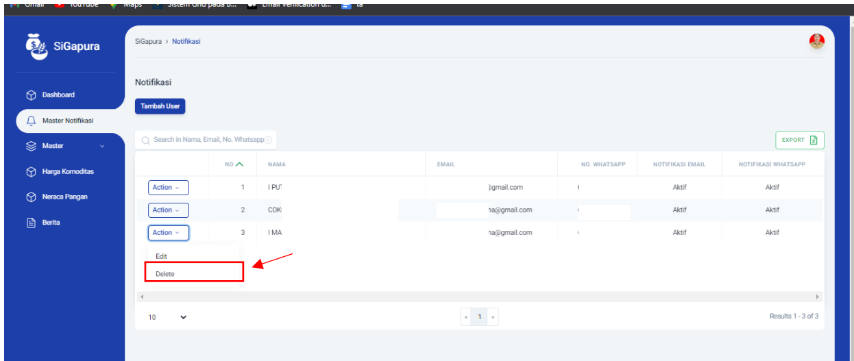
Gambar 3.8. Delete User
